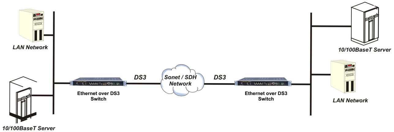
Remote LAN Connections over Optical Sonet/SDH Network
